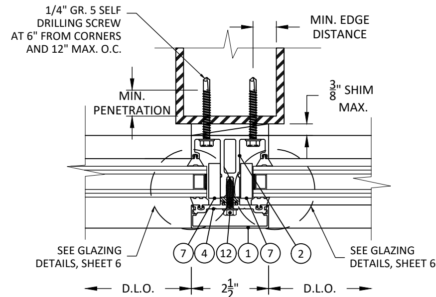
ANCHOR DETAIL ALUMINUM
