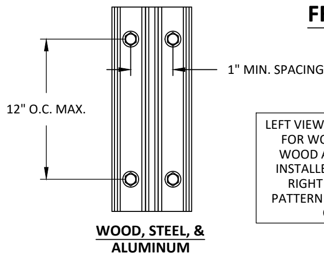
ANCHOR DETAIL WOOD
