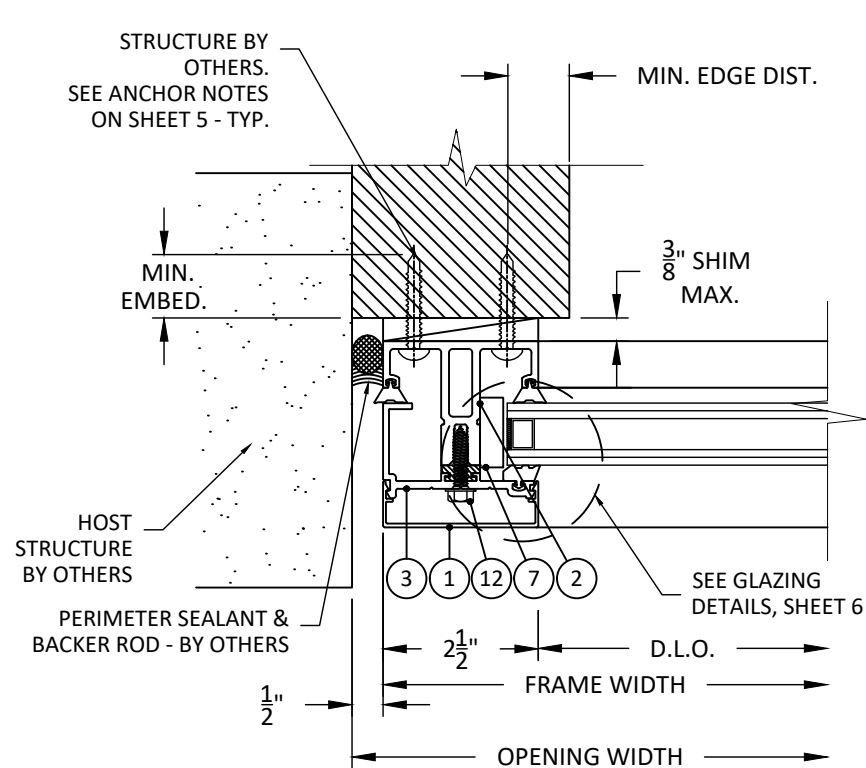
D 4 HORIZONTAL SECTION JAMB - INSULATING GLASS
