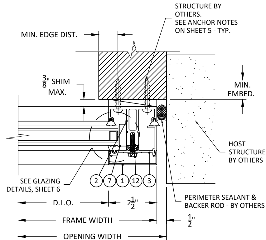
F 4 HORIZONTAL SECTION JAMB - INSULATING GLASS
